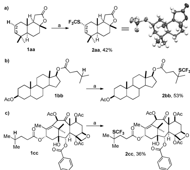
Scheme 3. Silver-mediated C(sp 3 )-H trifluoromethylthiolation reactions of natural products and natural-product derivatives. Reaction conditions: a) \text{AgSCF}_3 (2.5 equiv), \text{Na}_2\text{S}_2\text{O}_8 (4.0 equiv), \text{MeCN}/\text{H}_2\text{O}/\text{DCE} , 35 °C.
